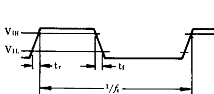
Fig. 4 Clock timing
